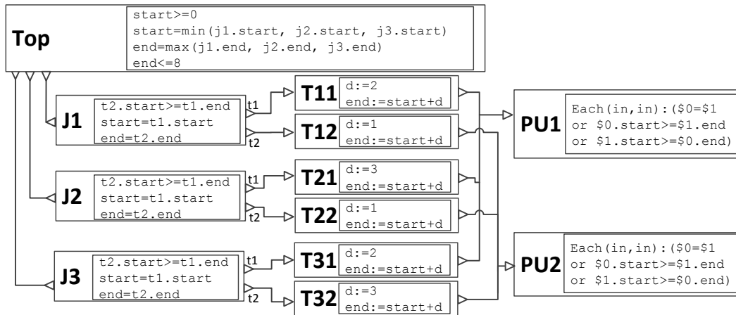
Fig. 5. CoDeL description of the De Moura's scheduling use case. The top component initializes three jobs (J1..J3), which each use two tasks each (T11..T32), which are mapped to two processing units.
