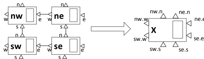
Fig. 7. Hierarchical composition of a 2x2 XGRID switch.
