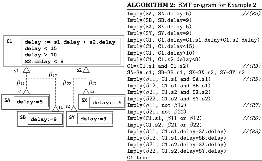
Fig. 4. Example 2.: Component C1 uses two sensor interfaces s1 and s2. For both types of sensor two alternative sensors are available, which results in four possible bindings ( \beta_{11} - \beta_{22} ). The assumptions in C1 allow the combination SB and SX (via \beta_{12} and \beta_{21} ) as the only conflict-free design..
