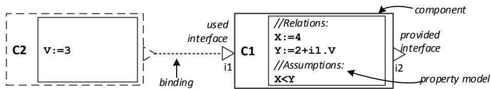
Fig. 2. Core elements of the component model: Component C1 has one used interface ( i1 ), one provided interface ( i2 ). Properties of C1 are described by two relations and one assumption. Connecting component (C2) using the i1 -interfaces sets the values of variables in scope of C1 ( i1.V=V of C2) so that the assumption ( X<Y ) can be satisfied.
