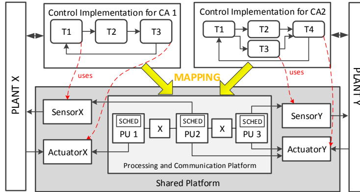
Fig. 9. Example for a mapping problem: Two control applications (CA1, CA2), implemented as sequential set of tasks should be mapped on shared processing units (PU1-3) and its interconnect network (X). Tasks need access to interfaces which can only be provided by a subset of the PUs (indicated by red arrows).
